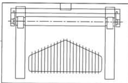
Curtain valve - external (above) and internal (below)
